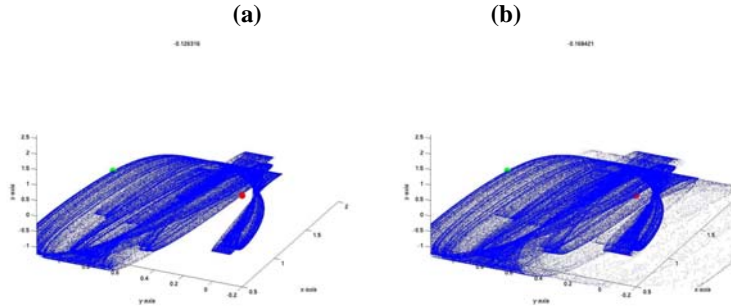
Figure 8: A numerical example of a heteroclinic bifurcation in three dimensions without tangencies. There are two saddle fixed points, p and q . (a) Prior to bifurcation, the attractor contains p but does not contain q . It is contained in the closure of a portion of U(q) . (b) At bifurcation, there is an explosion in which new points become part of the attractor. However, the density of the new part of the attractor is low.
