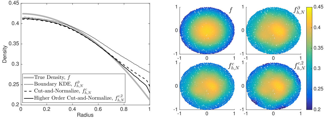
Fig. 3. Comparison of the boundary correction, cut-and-normalize method, and higher order cut-and-normalize method on the disk of Example 3.3. Left: Average value of each density estimation method as a function of radius after repeating the experiment of Example 3.3 10 times with independent data sets which shows the bias (variance error is averaged out). Notice that the higher order cut-and-normalize method f_{h,N}^{c,2} has similar bias on the boundary and the interior, which is order h^2 = 0.04 in each case. Right: A single realization of the experiment in Example 3.3 showing the true density and all three density estimates (note that the color scale is different than in Figure 2 to better show the differences in these estimates).
