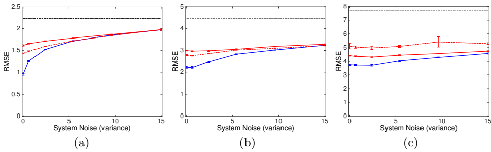
Fig. 4. Reconstructing the noisy Lorenz-63 x variable under increasing levels of dynamical noise. Observations of stochastic signal perturbed by Gaussian observational noise with variance (a) 5, (b) 20 and (c) 60 resulting in signal error level (dotted black line). Parametric filter (solid blue line), Kalman-Takens filter with 2 delays (solid red line) and Kalman-Takens filter with 4 delays (dotted red line) reconstruction accuracy shown. Error bars denote standard error over 5 realizations. As the amount of dynamical noise increases, the Kalman-Takens filter has performance very similar to the parametric filter, which has access to the full model.
