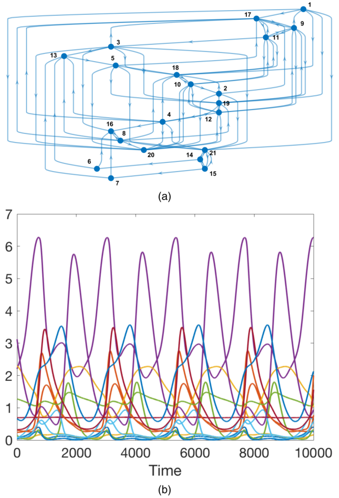
FIG. 5. (a) Network diagram representing the 21-variable differential equation of circadian rhythm model described in [23]. (b) The 21 traces show a periodic trajectory of the 21 variables of the regulatory network in (a).
