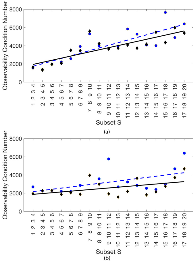
FIG. 4. (a) Mean observability condition number of the scale-free network, as a function of the four-member observation subsets S . Circles (dashed lines) denote nodes sorted by descending degree; diamonds (solid lines) denote nodes sorted by descending closeness centrality. (b) Same as (a), for the Erdős-Rényi network.
