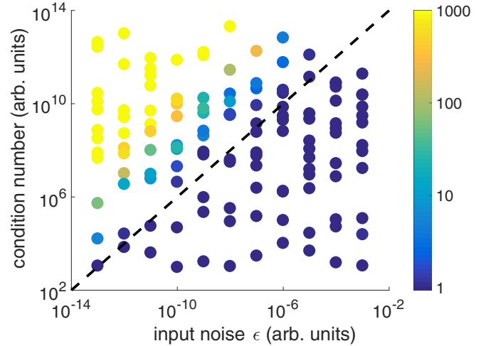
FIG. 7. Symbols are colored per estimates of \kappa_{S,X} and plotted versus the input noise and the condition number C of the Gauss-Newton iteration, for a completely observed network of random 2 \times 2 matrices. Trajectory lengths vary from 20 (lower symbols) to 240 (upper symbols). Calculations below the dashed line C = 10^{16}\sigma are reliable.
