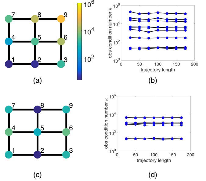
FIG. 1. Undirected network of nine nodes with dynamics, (5), and adjacency matrix A as shown. (a) Node X is shaded according to \kappa_{S,X} , where S = \{1, 2\} . (b) Estimates of \kappa_{S,X} in (a) as a function of the trajectory length. (c) Same as (a), but S = \{2, 8\} . (d) Estimates of \kappa_{S,X} in (c).
