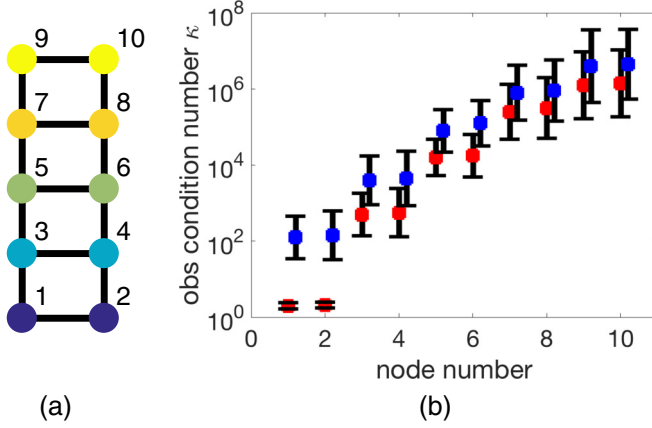
FIG. 2. (a) A network of 10 nodes with dynamics from (5). (b) Plot of \kappa_{S,X} for nodes 1–10 when observed at x coordinates of subset S = \{1, 2\} . Means and standard deviations for the x^j (left; red symbols) and y^j (right; blue symbols) variables are shown. Colors correspond to the color bar in Fig. 1.
