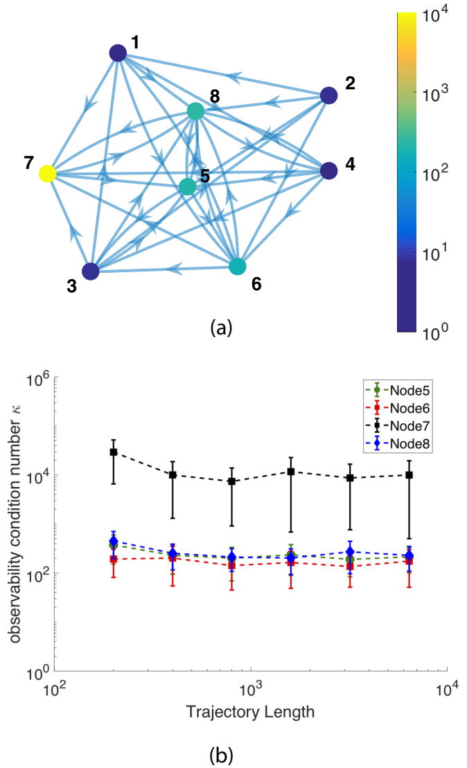
FIG. 3. (a) \kappa_{S,X} for the FitzHugh-Nagumo network. (b) Estimates of \kappa_{S,X} versus trajectory length. Although not obvious from the adjacency matrix, node 7 is more difficult to observe from the set S = \{1, 2, 3, 4\} than the remaining nodes.
