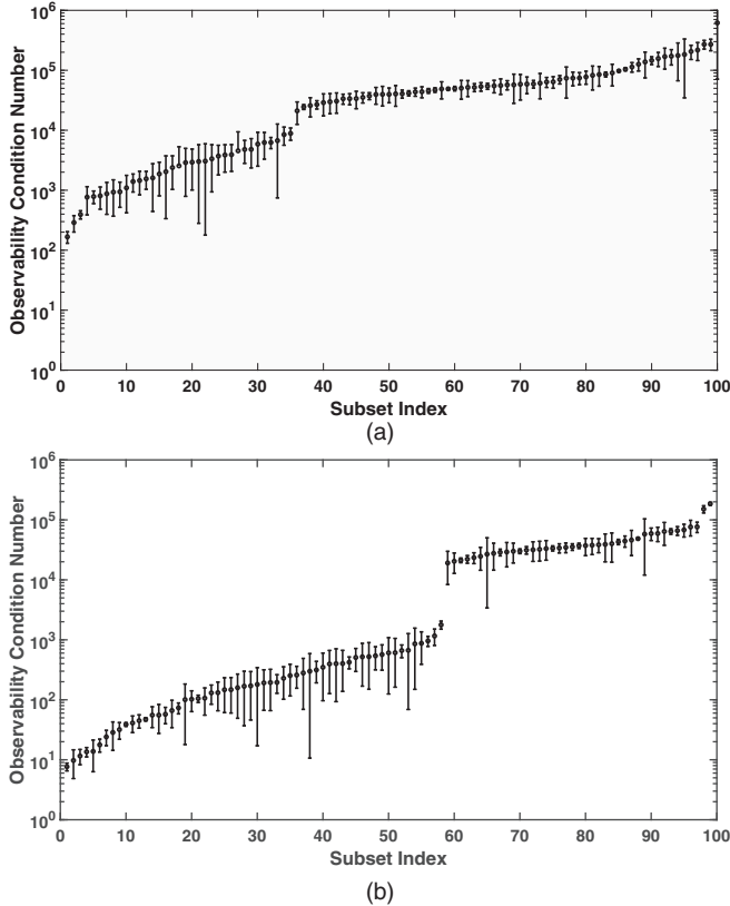
FIG. 6. Mean observability condition number \kappa_{S,X} for the 21-node regulatory network of [23], for the trajectory in Fig. 5(b). (a) A total of 100 subsets S of three nodes, chosen randomly, are compared. The subsets are sorted from left to right by increasing \kappa_{S,X} . There is a noticeable gap after the first 35 subsets. All subsets to the left of the gap contain either node 8 or node 16, corresponding to reactant RORc or Rorc, respectively. None of the subsets to the right of the gap contain either RORc or Rorc. (b) Average observability condition number \kappa_{S,X} for six-node subsets S along the horizontal axis. See the Supplementary Material [24] for identification of the three-node and six-node subsets, respectively.
