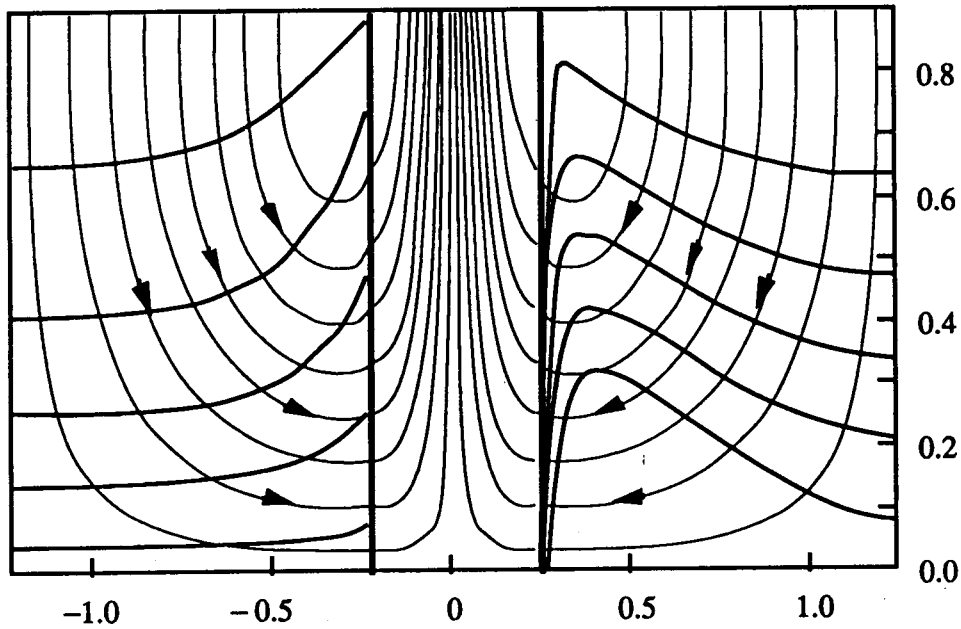
Figure 4. The thin lines show the streamlines through the mushy layer and up through a chimney (the central portion). Superposed on the left, in thicker curves, are isotherms. Superposed on the right are contours of solid fraction. The width of the chimney and the aspect ratio of the mushy layer are not to scale. The width of the chimney is inversely proportional to the cube root of the Darcy number \mathcal{H} and so is typically much narrower than its height.
