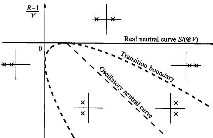
FIGURE 7. The character of the growth rates predicted by the conceptual model. The insets show the locations of the two normal-mode growth rates in the complex plane. The system is unstable when at least one of the roots has a positive real part. The diagram shows the neutral curves for real and oscillatory modes and the transition boundary where two real modes combine to form a complex-conjugate pair.
