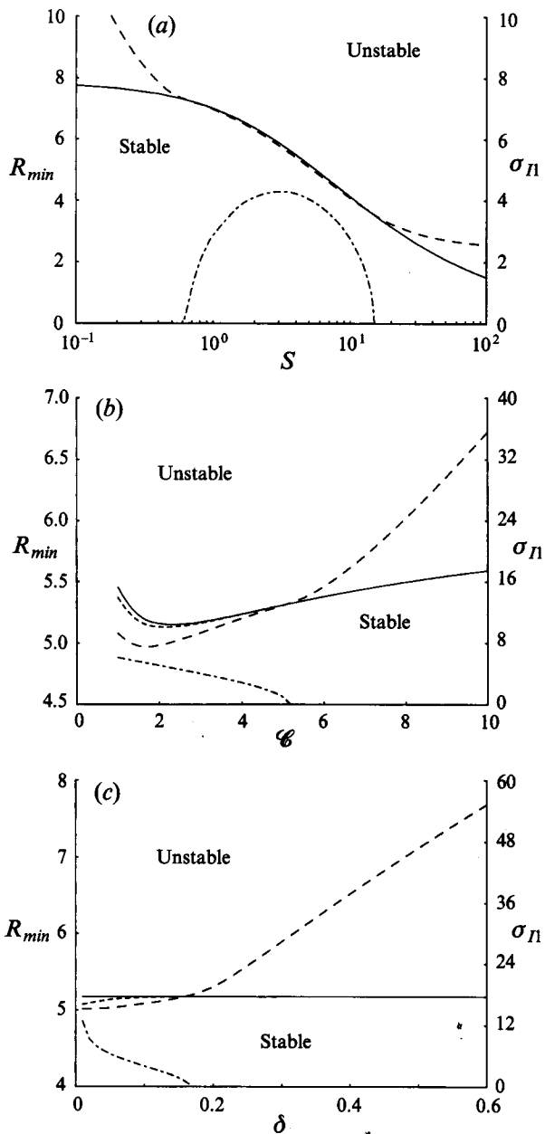
FIGURE 5. The critical Rayleigh numbers as they vary with the dimensionless parameters S , \mathcal{G} and \delta , with K_1 = 3 . The solid curves indicate the critical Rayleigh numbers for the neutrally stable real mode, the long-dashed curves indicate the critical Rayleigh numbers for the neutrally stable oscillatory mode, and the short-dashed curve represents the transition boundary between real and oscillatory modes. The basic-state solution is stable (unstable) below (above) the curves. Also indicated is the frequency \sigma_{11} (dashed-dotted curve) along the oscillatory branch. Note that the ranges in which the frequency is zero correspond to those cases where the oscillatory mode has an endpoint minimum and that within these ranges the transition boundary coincides with the critical curve for the oscillatory mode. (a) The variations with S with \delta = 0.1 and \mathcal{G} = 3 . Note that the transition boundary is not resolved on the scale of this figure but lies just below the critical curve for the real mode for 0.6 < S < 15 approximately and coincides exactly with the critical curve for the oscillatory mode outside this range. (b) The variations with \mathcal{G} with \delta = 0.1 and S = 5 . (c) The variations with \delta with S = 5 and \mathcal{G} = 3 . Note that, to the order we have shown, the real mode is independent of the mushy-layer thickness \delta .
