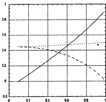
Figure 10 Corner Coordinates versus R_c for A = 0.5 and \rho = 1.05 . — \phi , --- Z_c , · · · Z_t . The extrapolation of the angle to R_c = 0 shows that a dimple can form.
