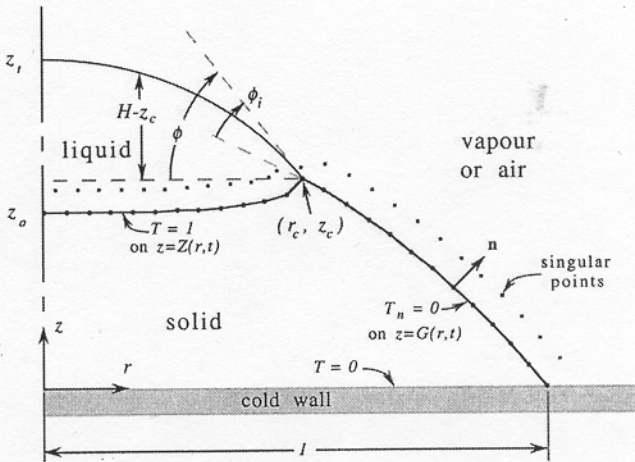
Figure 2 Problem schematic. All variables are dimensionless. In particular, the wetted drop radius is scaled to unity.
