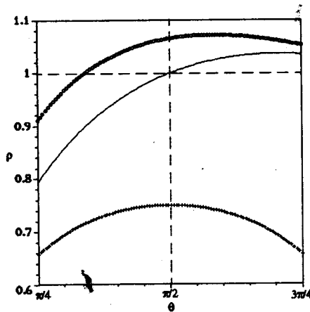
Figure 5 Cusp angle formation as a function of density ratio. The curve made of closely spaced plus signs is the flat interface model and is identical to a portion of the dashed line of figure 4 in Anderson et al. (1996). The solid line and that line composed of circles are for the spherically-shaped interface with growth angle \phi' of 0 and 10 degrees, respectively. Note that conical peaks are predicted when \theta < \pi/2 and conical dimples are predicted for \theta > \pi/2 . For the case with \phi' = 0 (the fixed contact line condition), this transition from dimples to peaks occurs exactly at \rho = 1 .
